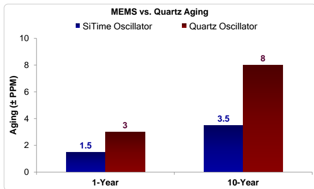
Figure 219. Aging Comparison [2]
