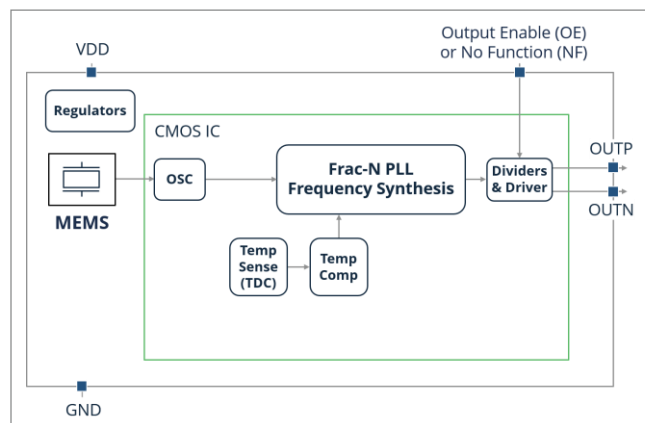
Figure 1. SiT9396 Block Diagram
