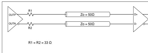
Figure 32. Low-power HCSL Termination
