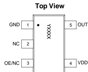
Figure 1. Pin Assignments
