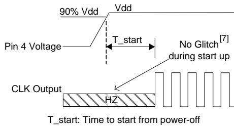
Figure 3. Startup Timing (OE/ \overline{ST} Mode)
