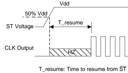
Figure 4. Standby Resume Timing ( \overline{ST} Mode Only)
