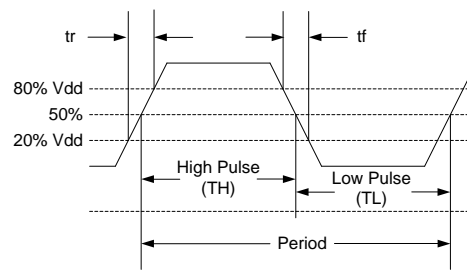
Figure 2. Waveform
