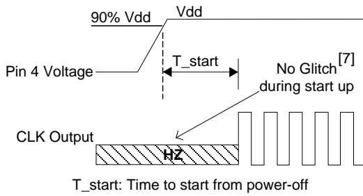
Figure 2. Startup Timing
