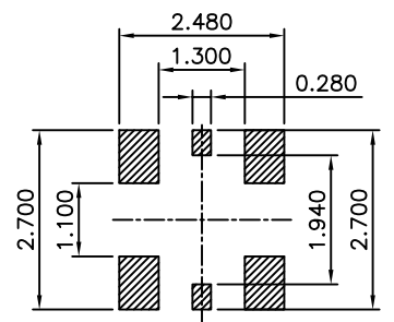
Recommend Stencil Mask Pattern (Mask Thickness 0.08mm)
