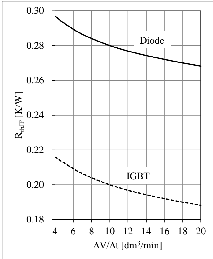
Fig 11. Thermal Impedance
