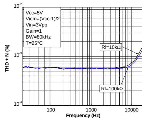
Figure 19. Distortion + noise vs. frequency
