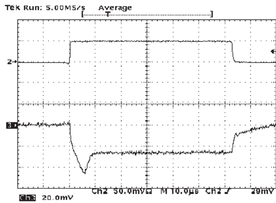
Figure 15. Load transient ( C_O = 10 \mu\text{F} )
