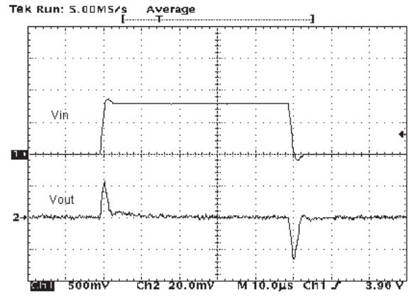
Figure 14. Line transient ( t_r = t_f = 1 \mu\text{s} )
