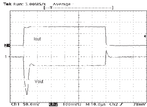
Figure 16. Load transient ( C_O = 4.7 \mu\text{F} )
