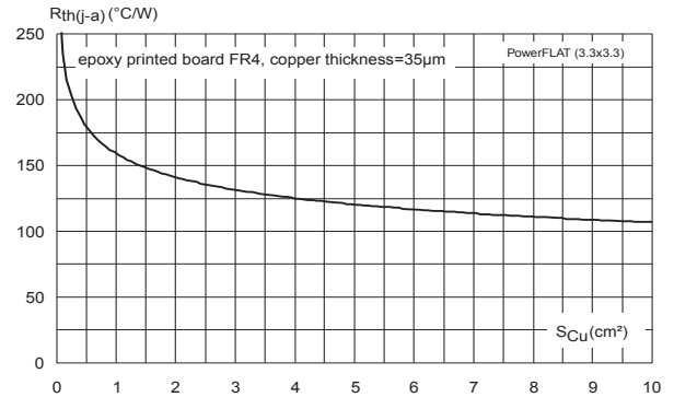
Figure 8. Thermal resistance junction to ambient versus copper surface under tab
