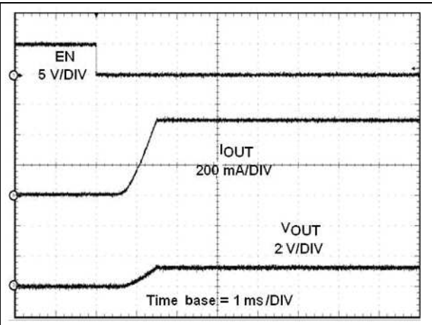
Figure 16. OC protection at V_{OUT} = 5.0\text{ V} (STMPS2141/2151 - details)
