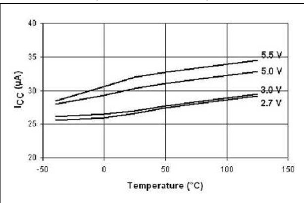
Figure 20. I_{CC} vs. temperature (disabled) (STMPS2141/2151)
