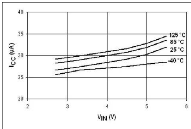
Figure 19. I_{CC} vs. V_{IN} (disabled) (STMPS2141/2151)
