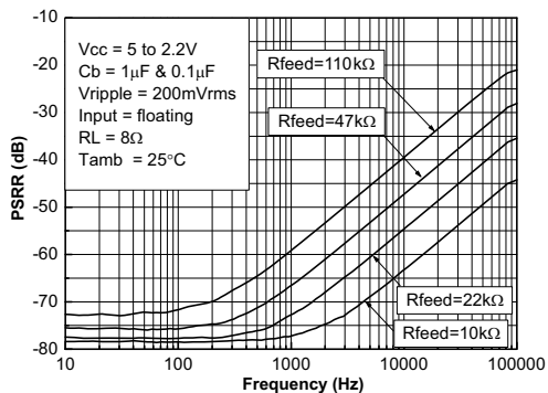
Figure 19. Power supply rejection ratio (PSRR) vs feedback resistor
