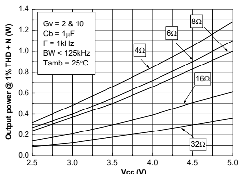
Figure 20. Pout @ THD + N = 1% vs supply voltage vs RL
