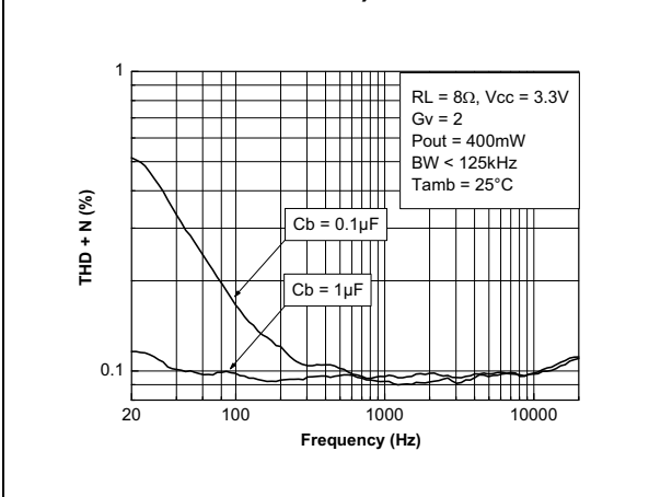
Figure 71. THD + N vs frequency (Pout= 400 mW)
