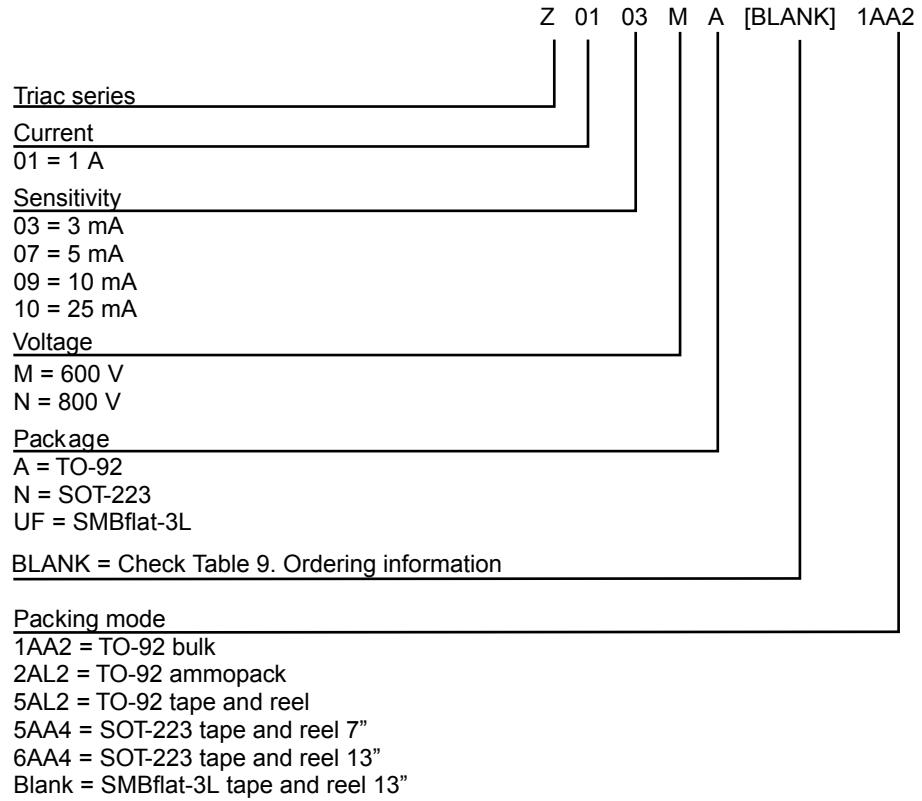
Figure 19. Ordering information scheme
