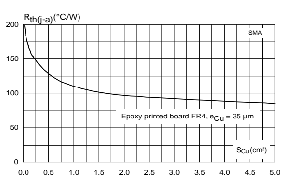
Figure 12: Thermal resistance junction to ambient versus copper surface under each lead (typical values)
