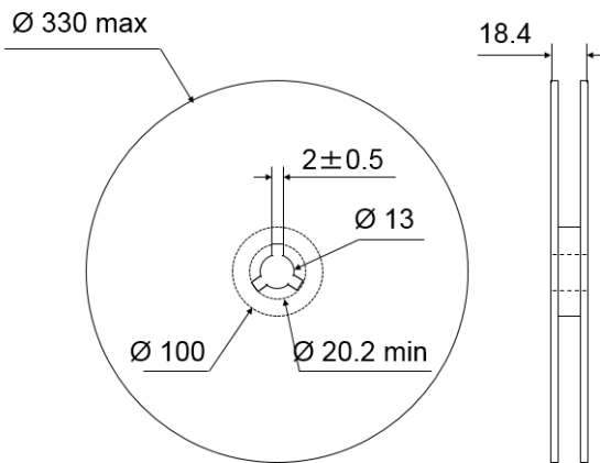
Figure 18. 13" reel dimension values
