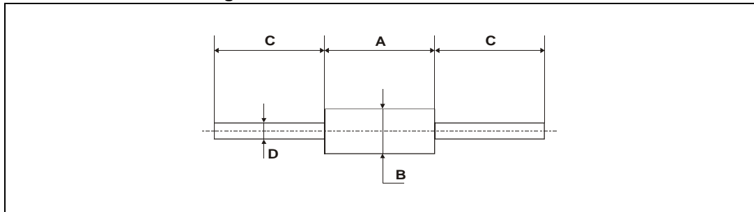
Figure 26. DO-15 dimension definitions
