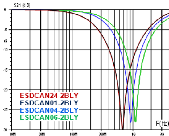
Figure 13. S21 attenuation
