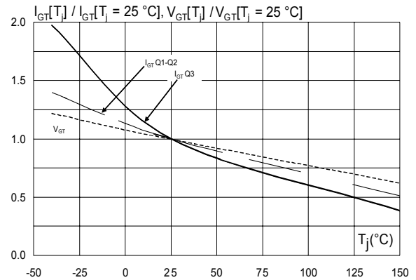
Figure 8. Relative variation of gate trigger current and gate voltage versus junction temperature (typical values)
