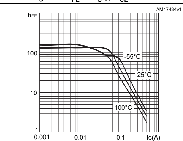
Figure 3. h_{\text{FE}} vs. I_{\text{C}} @ V_{\text{CE}} = 10\text{ V}
