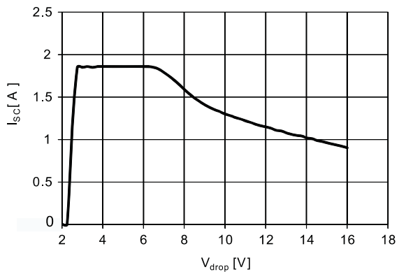
Figure 9: Short-circuit current vs. dropout
