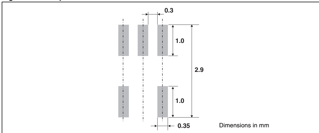
Figure 13. Footprint dimensions
