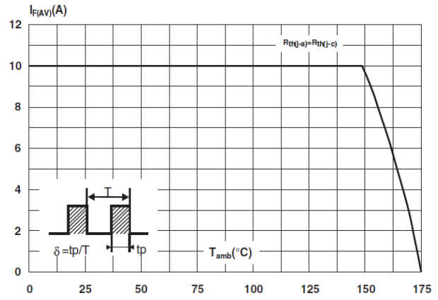
Figure 2. Average forward current versus ambient temperature (δ = 0.5)
