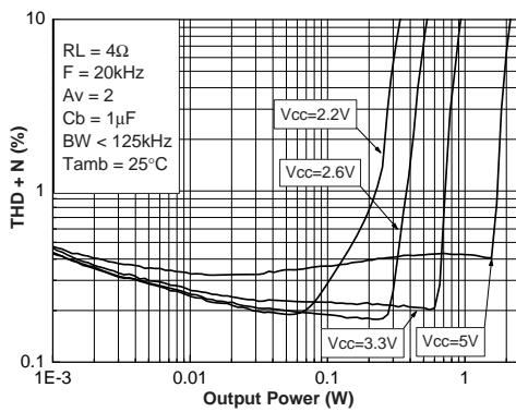
Figure 46. THD + N vs. output power F = 20 \text{ kHz}
