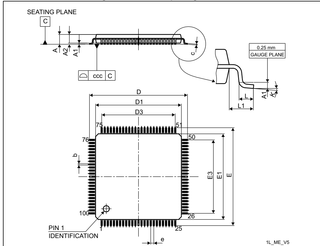
Figure 64. LQFP100 package outline
