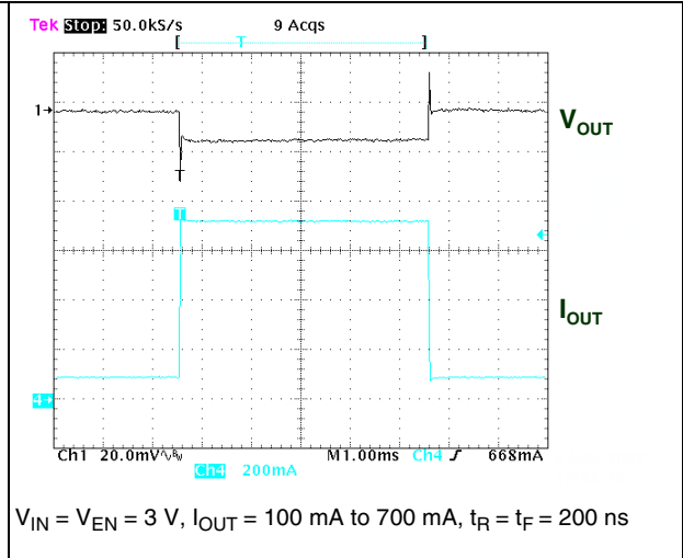
Figure 23. Load transient
