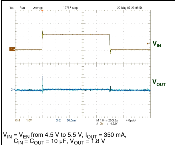
Figure 22. Line transient
