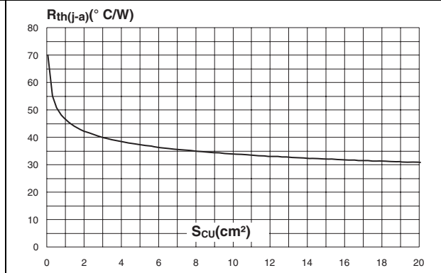
Figure 10. Thermal resistance junction to ambient versus copper surface under each tab (Epoxy printed circuit board FR4, e CU = 35 μm) for D 2 PAK
