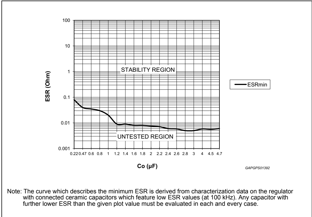
Figure 15. Stability region
