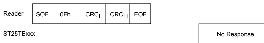
Figure 32. Completion frame exchange between reader and ST25TB512-AC
