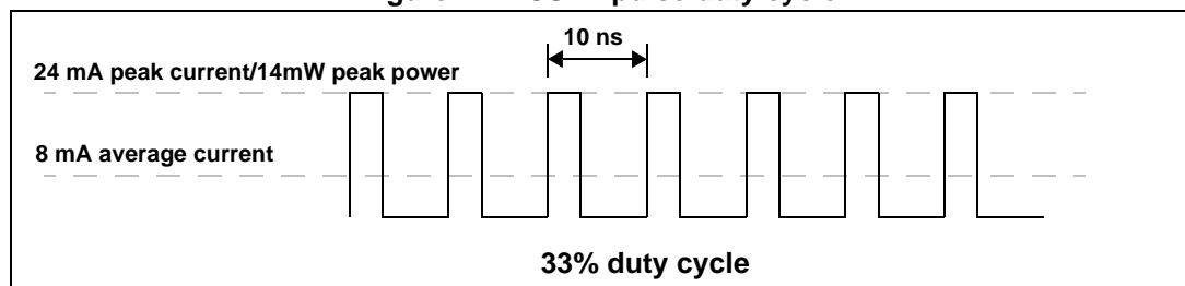
Figure 27. VCSEL pulse duty cycle
