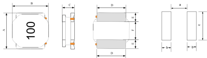
Recommended PCB pattern
