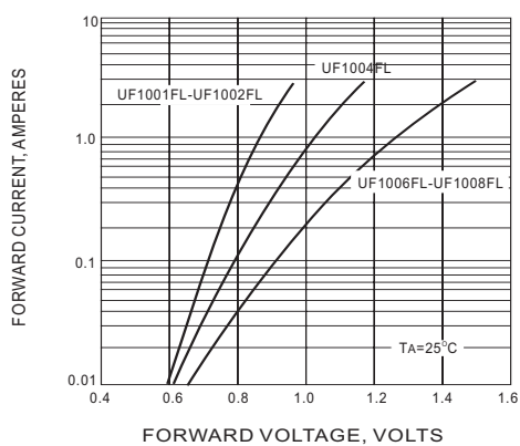
Fig.3 FORWARD CHARACTERISTICS
