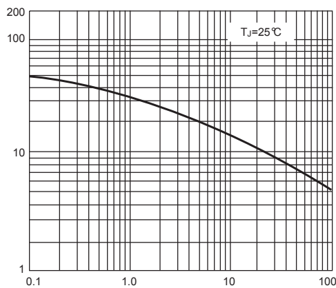
FIG. 5-TYPICAL JUNCTION CAPACITANCE
