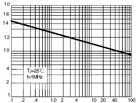
FIG.5-TYPECAL JUNCTION CAPACITANCE
