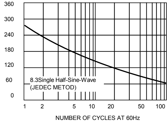
FIG.2-MAXIMUM NON-REPETITIVE SURGE
