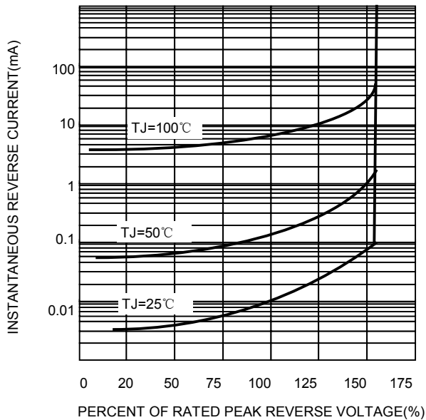
FIG.3-TYPICAL REVERSE CHARACTERISTICS
