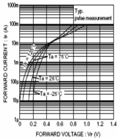
Fig. 1 Forward characteristics
