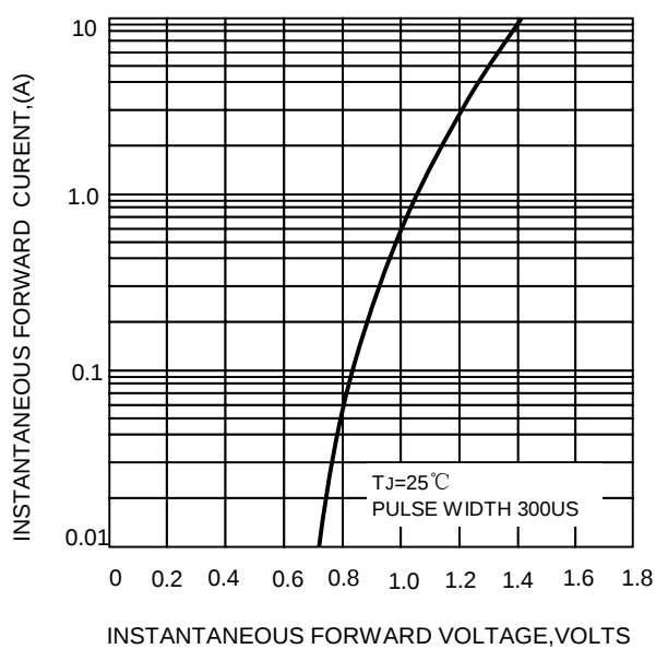
FIG.3-TYPICAL FORWARD CHARACTERISTICS
