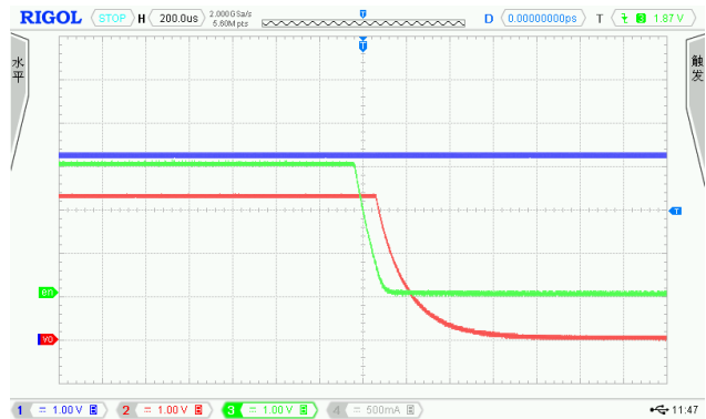
EN=3V to 0V, I OUT =10mA
