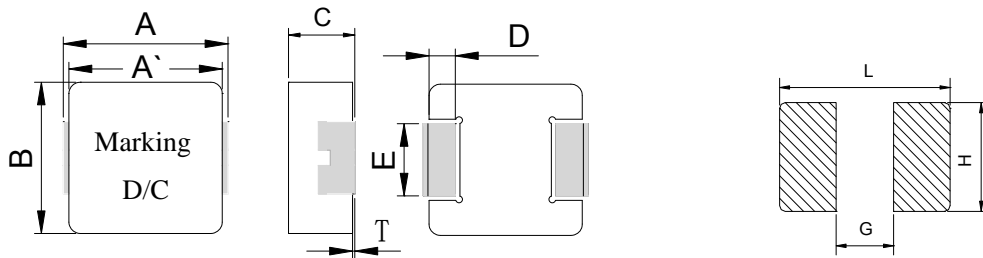
Recommended PC Board Pattern
