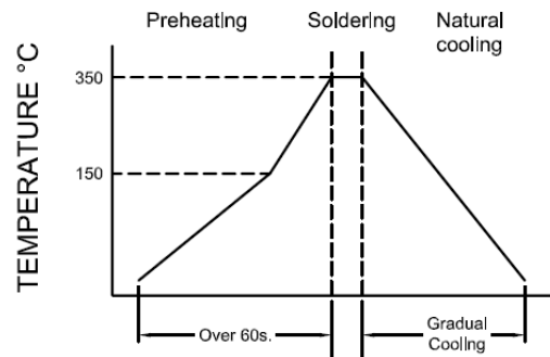
Iron Soldering times: 1 times max
