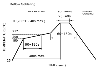
Reflow times: 3 times max Fig.1
