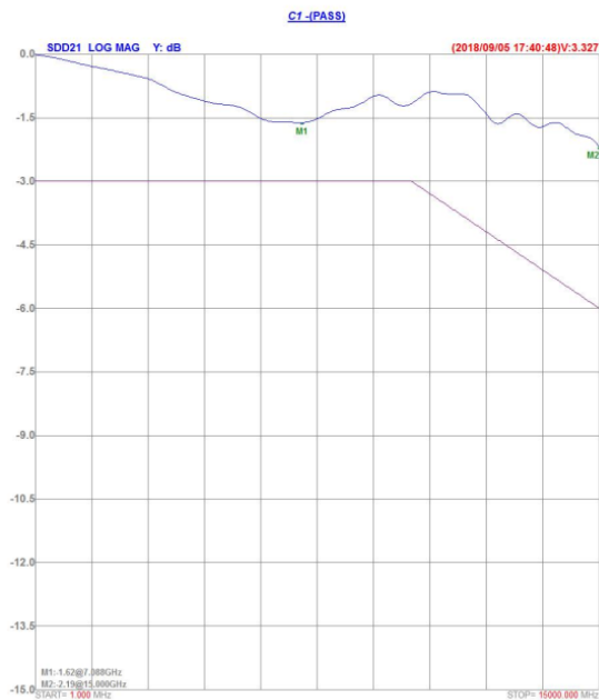
HSF2012F2SV-300T04-H USB3.1 Choke Insertion Loss Graphic result
