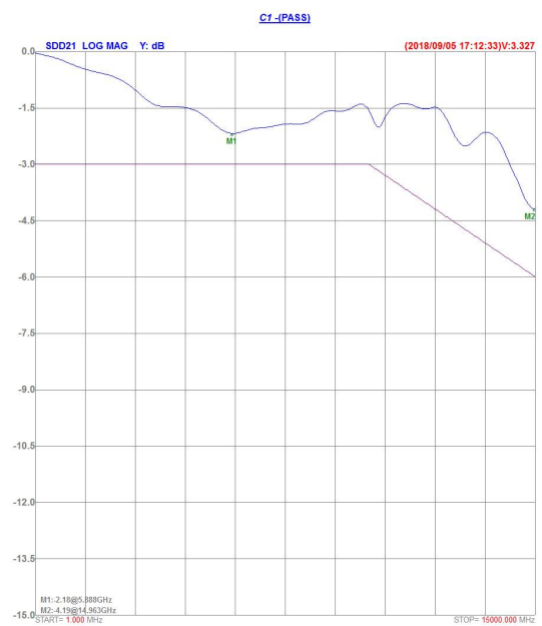
HSF2012F2SV-600T03-H USB3.1 Choke Insertion Loss Graphic result
