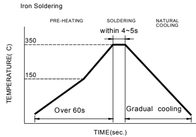
Iron Soldering times: 1 times max Fig.2
