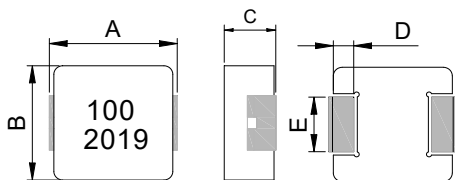
leadframe
