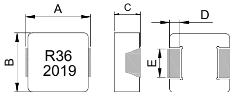
non-leadframe
