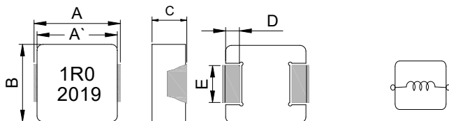
non-leadframe
