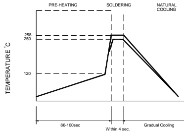
Figure 2. Wave Soldering
