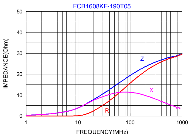
■ Impedance-Frequency Characteristics
