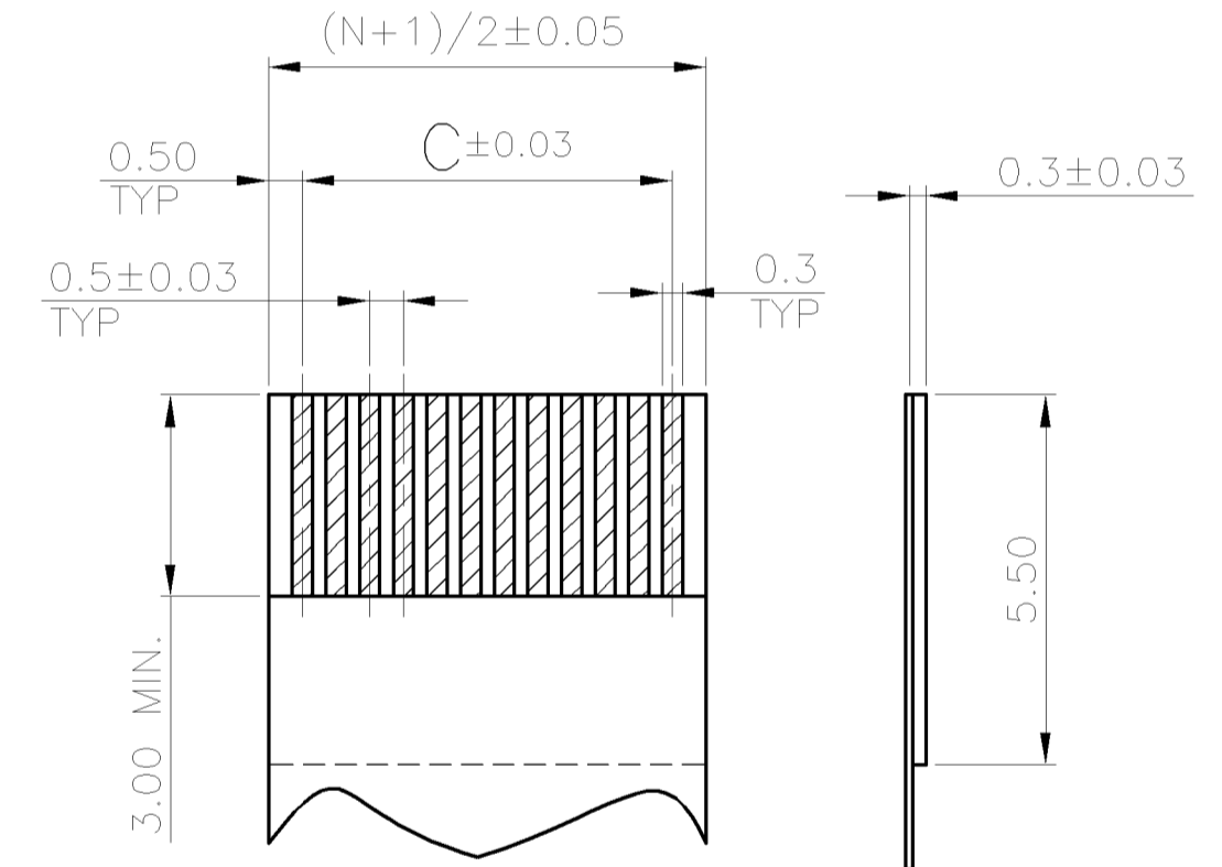
RECOMMENDED FPC/FFC LAYOUT (N = NO. OF CONTACTS)
