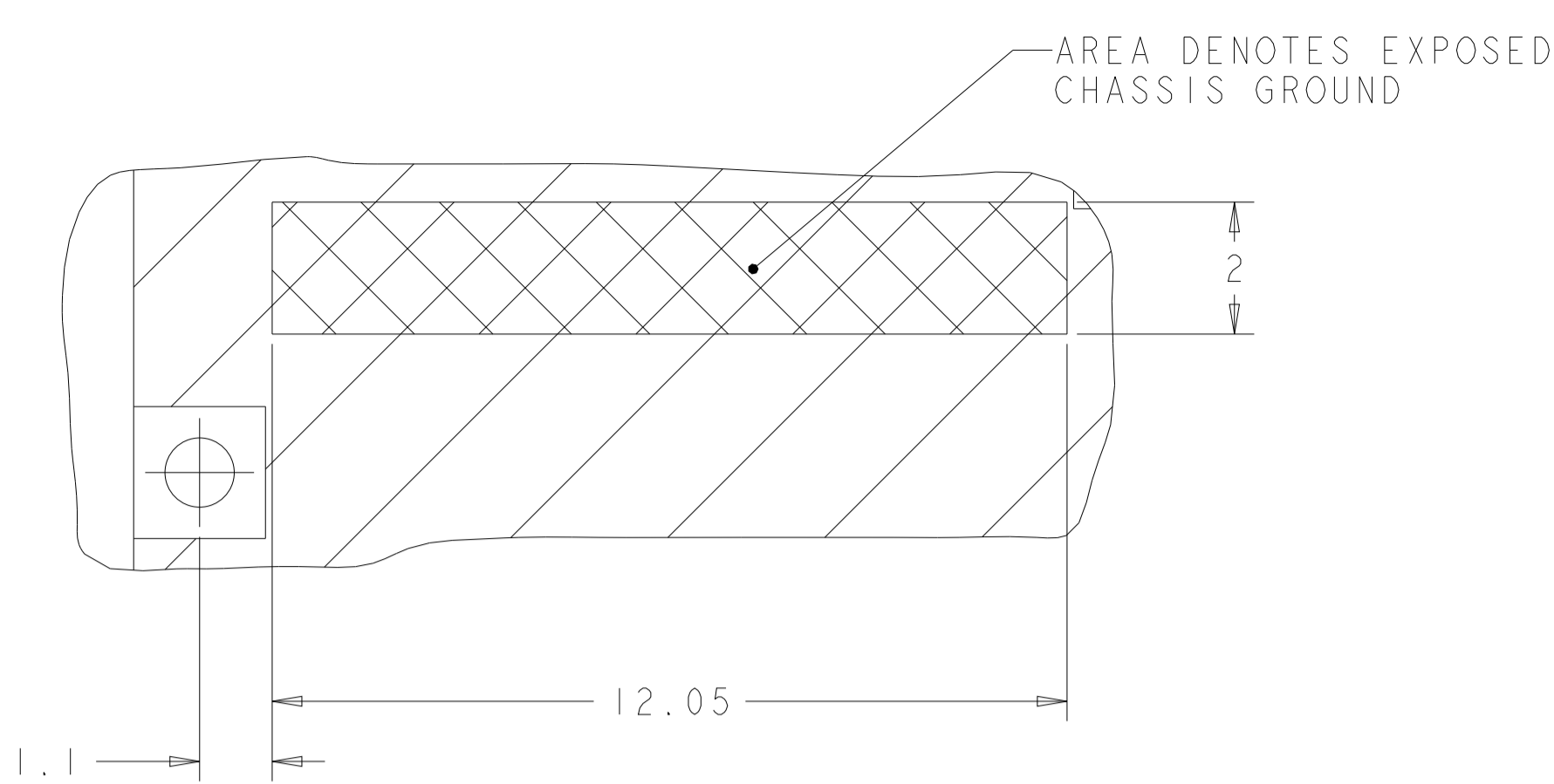
DETAIL A 4X INDIVIDUALLY SCALE 10:1
