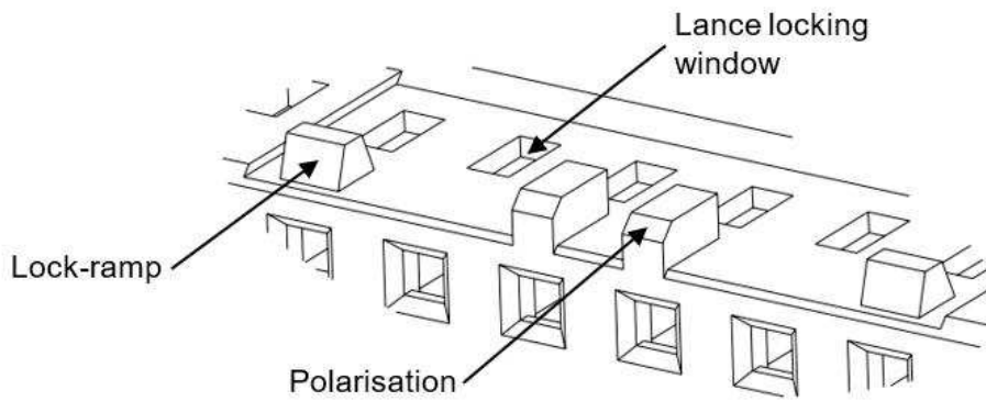
Housing – with Locking ramp
