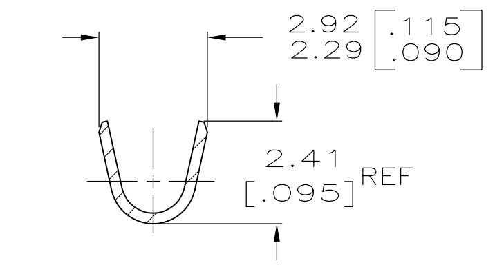
SECTION C-C SCALE 8:1
