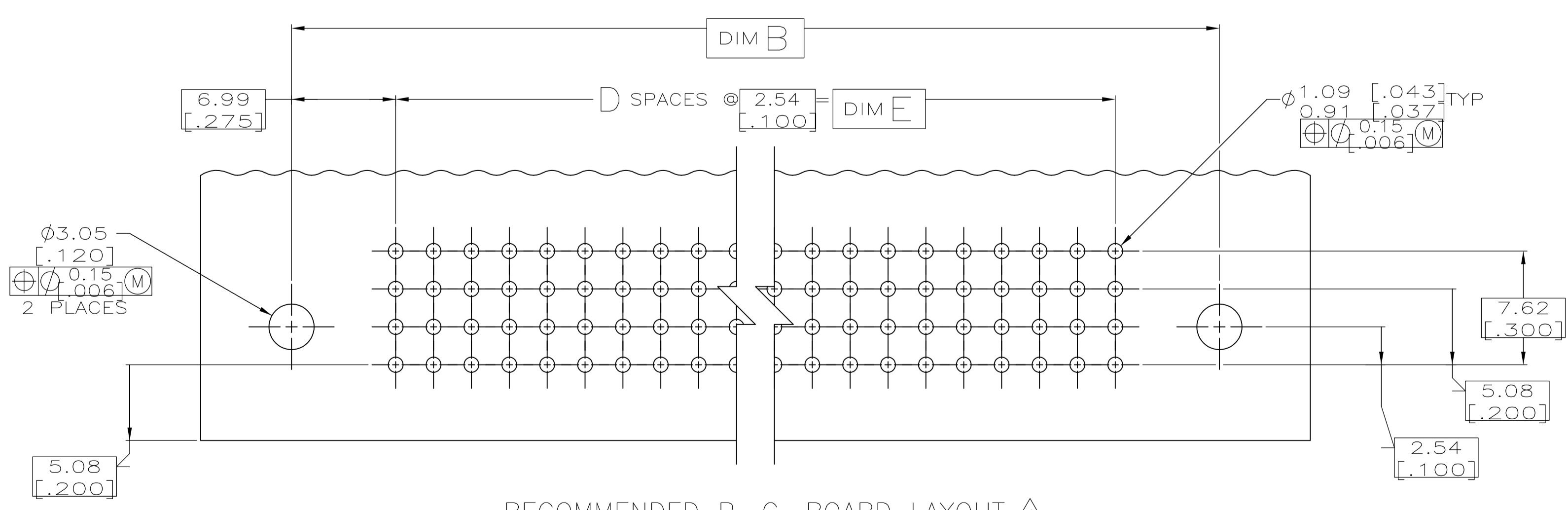
RECOMMENDED P. C. BOARD LAYOUT △4
